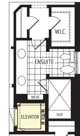
GROUND FLOOR (w/Elevator) PARTIAL PLAN OPT. ENSUITE W/BIDET
