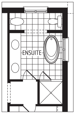
SECOND FLOOR PARTIAL PLAN OPT. ENSUITE W/BIDET
